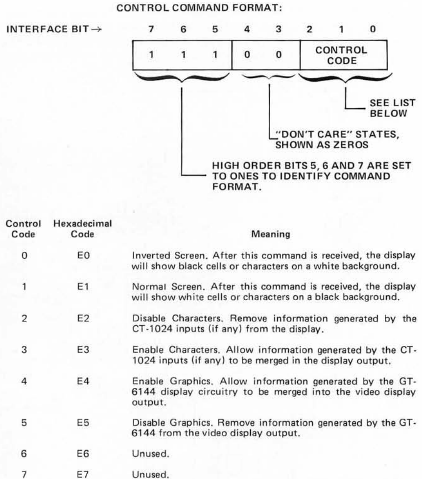
Figure 2: Data Formats for the Control Commands. The unused states of the vertical command format described in figure 1 are used to perform control operations. The control format and operations are shown here. Note that in the program of listing 1, the contents of bits 3 and 4 are assigned zero value arbitrarily since they are "don't care" inputs in control commands.
