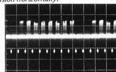
Photo 15: Test point 15, video output, 0.5 V per division vertically, 100 \mu s per division horizontally.
